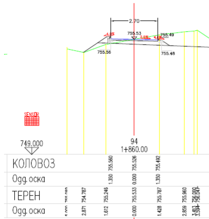
Figure 3 Cross-section of the bicycle track
